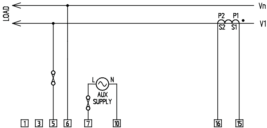
Figure 4-5 Single Phase
