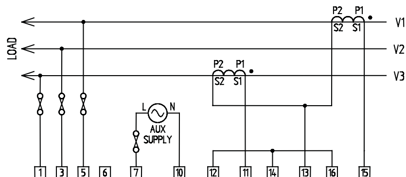
Figure 4-2 3-Phase 3-Wire 2CTs
