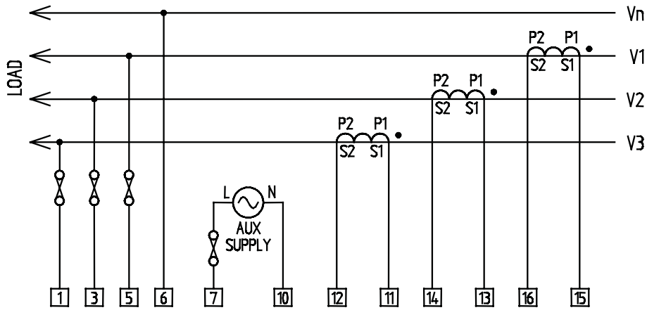
Figure 4-4 3-Phase 4-Wire (See Note 2)
