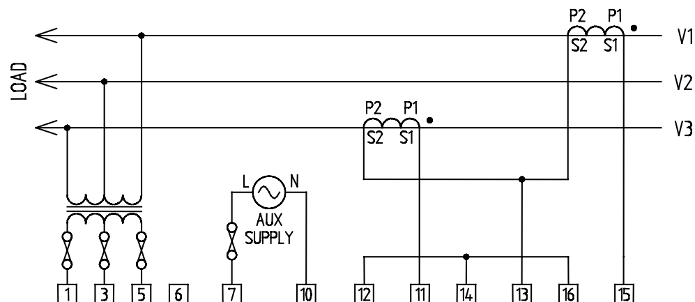
Figure 4-6 3 Phase 3 Wire Using Potential Transformers (2CTs)
