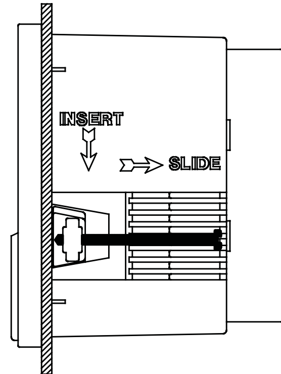
Figure 4-1 Fitting The Meter in a Panel
