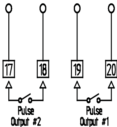
Figure 2.1 Pulse Output Connection
