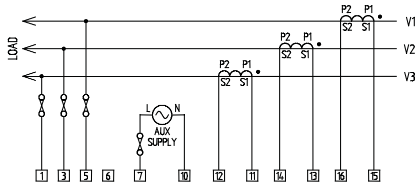
Figure 4-3 3-Phase 3-Wire 3CTs (See Note 2)
