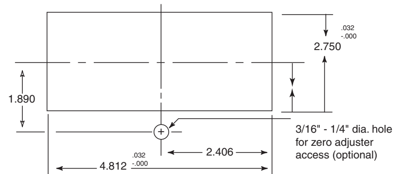
Figure 1. Drilling Template
