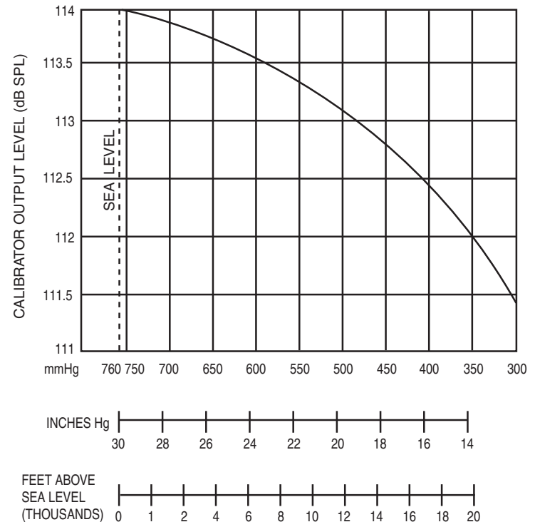
Figure 3-2. Effect of Elevation Upon Calibrator Output
