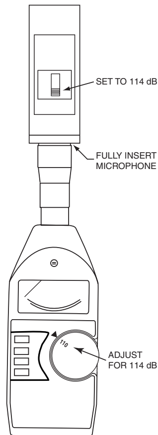
Figure 3-3. Sound Level Meter Calibration.
