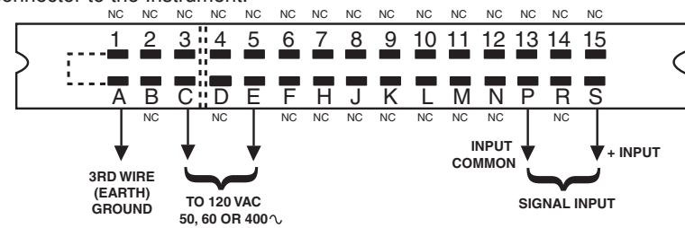
Figure 3. Model 2865, Connector Wiring
