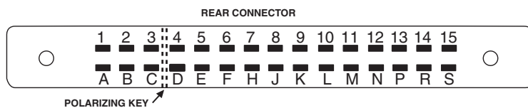
Figure 5. Rear Connector
