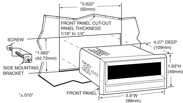
Figure 2. Panel Mounting and Cut-Out Dimensions
