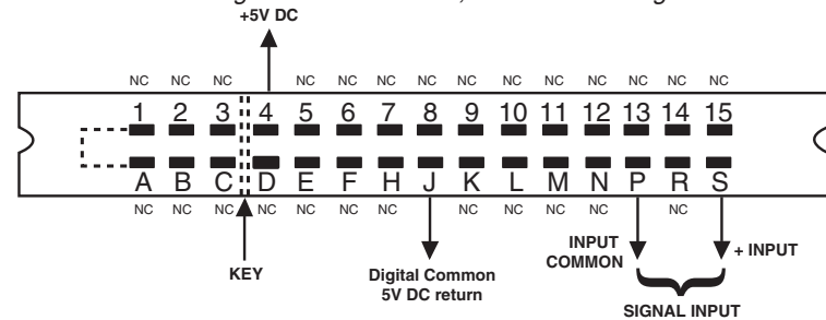
Figure 3. Model 2865, Connector Wiring
