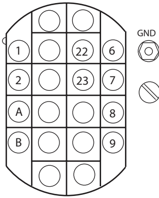
REAR VIEW OF HEADER
